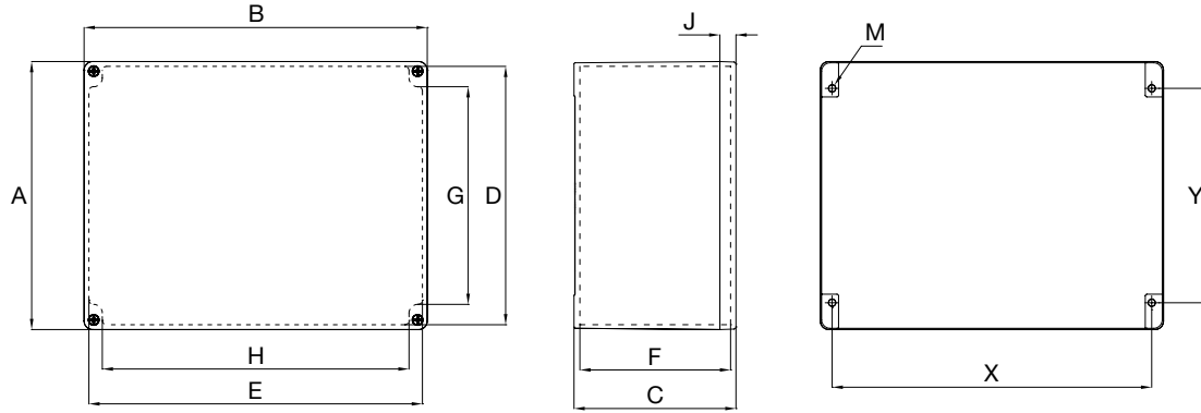
Dimensions in Millimeters (Inches) ①
